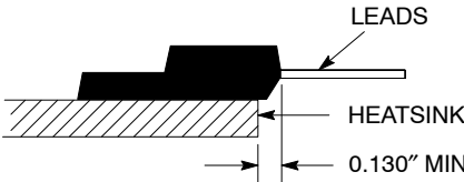
Figure 14. Mounting Position for Isolation Test
